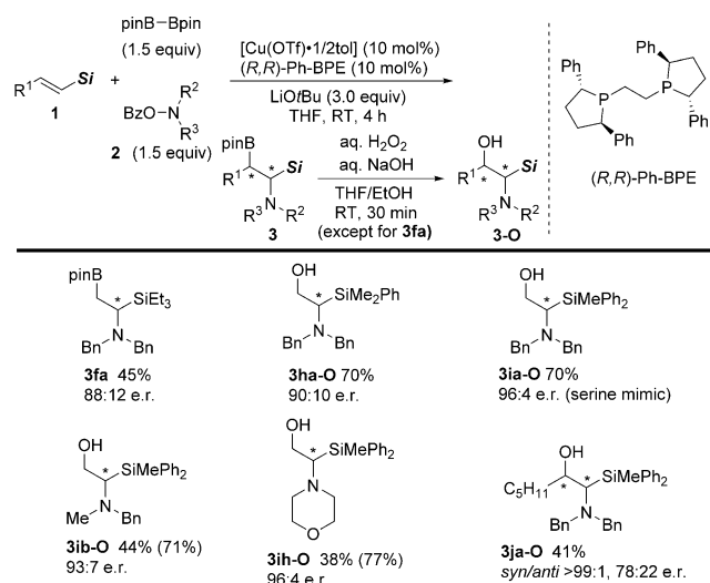
Scheme 6. Catalytic enantioselective aminoboration of vinylsilanes. 1 H NMR yield in the pinB form is in parentheses.
