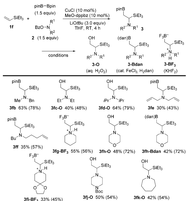
Scheme 4. Catalytic aminoboration with various hydroxylamines 2 . Isolated yields are given. 1 H NMR yield in the pinB form is in parentheses. See the Supporting Information for detailed conditions of the derivatization of the Bpin moiety. Boc = tert -butoxycarbonyl.
