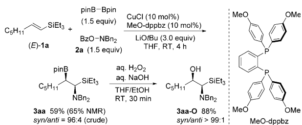
Scheme 2. Optimal conditions for copper-catalyzed aminoboration of vinylsilane ( E )- 1a and subsequent H 2 O 2 -promoted oxidation. Bn = benzyl.
